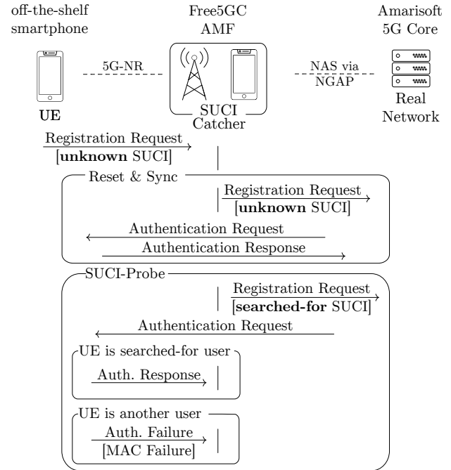
Figure 3: Attack Phase: Modified AKA-Linkability attack with an additional reset-step that enables repetition: our UE answers more than 500 SUCI-Probes in 60 seconds.
